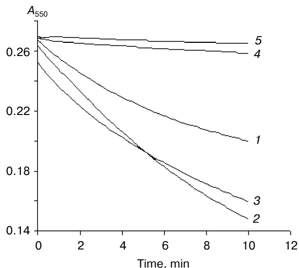
Fig. 2. Kinetics of xanthine oxidase-mediated DCPIP reduction in the presence of xanthine (1), allopurinol (2), and the following allopurinol-based inhibitors: 3) 4-amino-6-mercaptopyrazolo-3,4-d-pyrazolopyrimidine; 4) 4-mercapto-1H-3,4-d-pyrazolopyrimidine; 5) 4-amino-6-hydroxy-3,4-d-pyrazolopyrimidine. The concentration of each compound used was 10 \mu\text{M} . DCPIP concentration was fixed at 15 \mu\text{M} .
