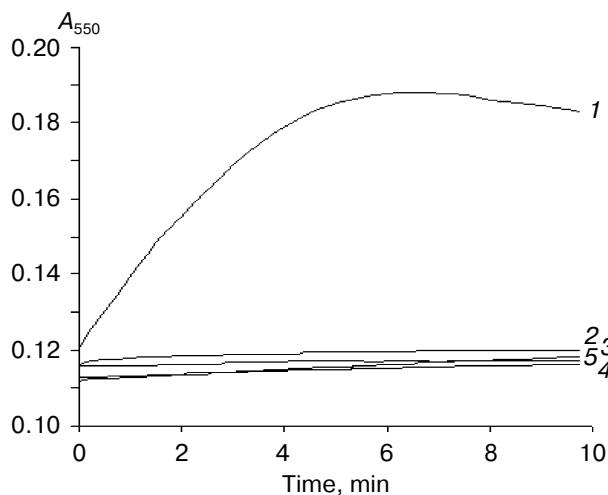
Fig. 3. Kinetics of xanthine oxidase-mediated superoxide formation in the presence of xanthine (1), allopurinol (2), and the following allopurinol-based inhibitors: 3) 4-amino-6-mercapto-3,4-d-pyrazolopyrimidine; 4) 4-mercapto-1H-3,4-d-pyrazolopyrimidine; 5) 4-amino-6-hydroxy-3,4-d-pyrazolopyrimidine. The concentration of each compound used was 10 \mu M. Cytochrome c concentration was fixed at 15 \mu M.
